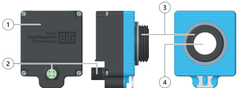
Label Adapter cartridge
