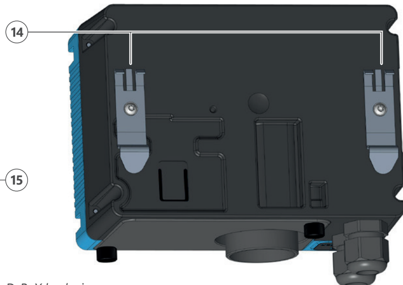
D-ReX back view
