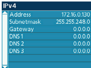
State IPv4
