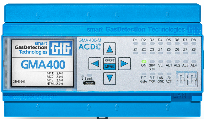
GMA400 – with Modbus TCP and web access through ethernet
